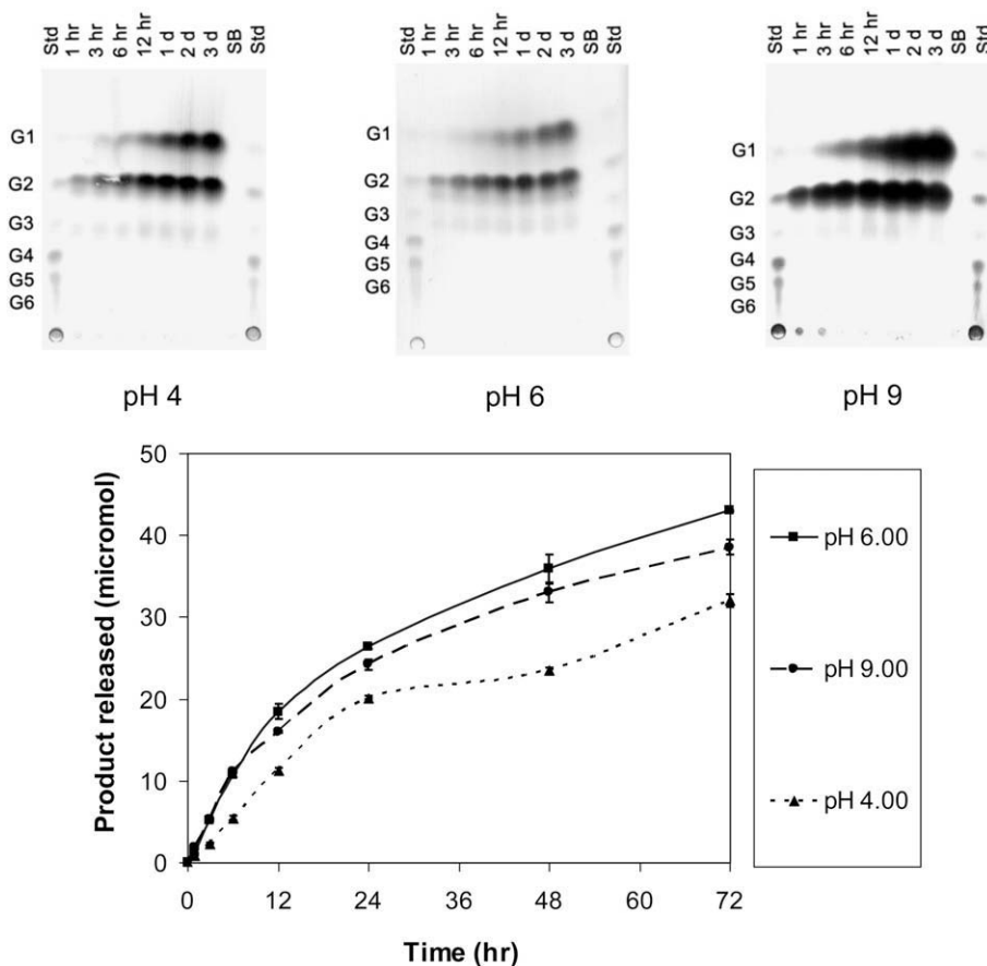
Fig. 5. Analysis of reaction products in various buffers. Upper panel illustrates TLC analysis of colloidal chitin hydrolysis by B. licheniformis ChiA1 at three different buffers. The hydrolytic reaction was carried out at 50 °C for up to 3 days in the presence of 30 mg colloidal chitin and 50 µg enzyme in 800-µl reaction volume. The reaction products after incubation for 1 h, 3 h, 6 h, 12 h, 1 day, 2 day and 3 day are shown. Std: a standard mixture of G1–G6; SB: substrate blank; hr: hour; d: day. The contrast and brightness of the pictures were enhanced by Image J software (Abramoff et al., 2004). Quantitative analysis of products released at various time points, determined by DNS method (Miller, 1959), is depicted in the lower panel.
