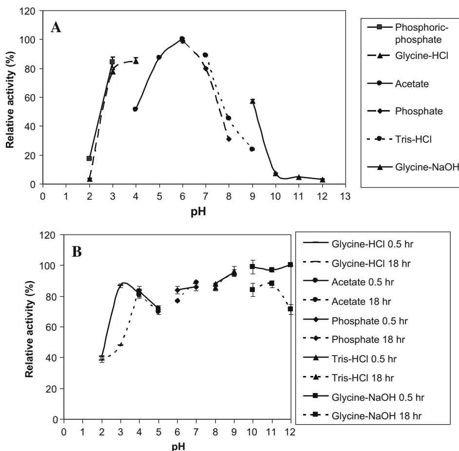
Fig. 2. Effect of pH on catalytic activity. (A) The optimal pH was determined at 37^{\circ}\text{C} in 100 mM of different buffers as indicated under the standard assay condition. (B) The pH stability was determined by measuring the residual activity of ChiA after incubation at various pHs at 20^{\circ}\text{C} for 30 (solid line) min or 18 h (broken line) without substrate.
